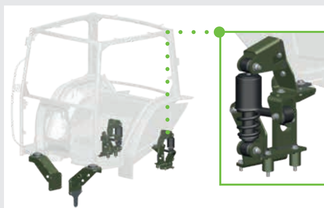
Mechanical cab suspension.
